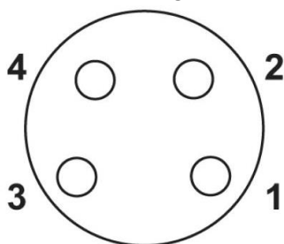
Pin assignment M8-jack, 4-pol, A-coding
