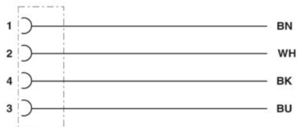
Pin assignment from M8-jack
