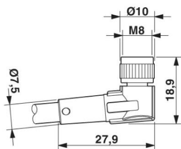
Jack M8 x 1, angled
