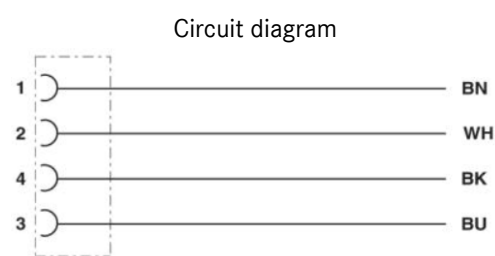
Pin assignment M8-jack
