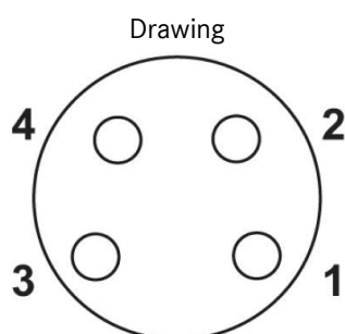
Pin assignment M8-jack, 4-pol, A-coding
