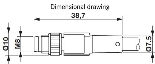
Plug M8 x 1, straight
