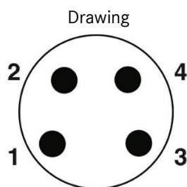
Pin assignment M8-plug, 4-pol, A-coding
