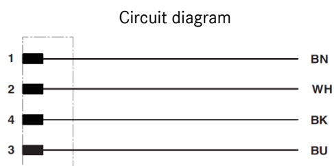
Pin assignment M8-plug
